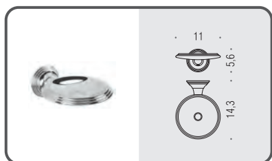
B3301 Porta sapone Soap dish holder
