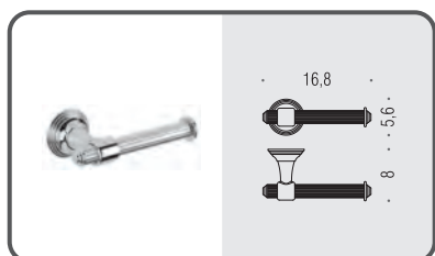
B3308 Porta rotolo Paper holder
